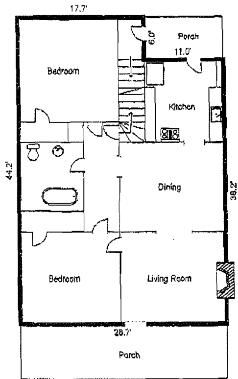
FIRST FLOOR LEVEL
